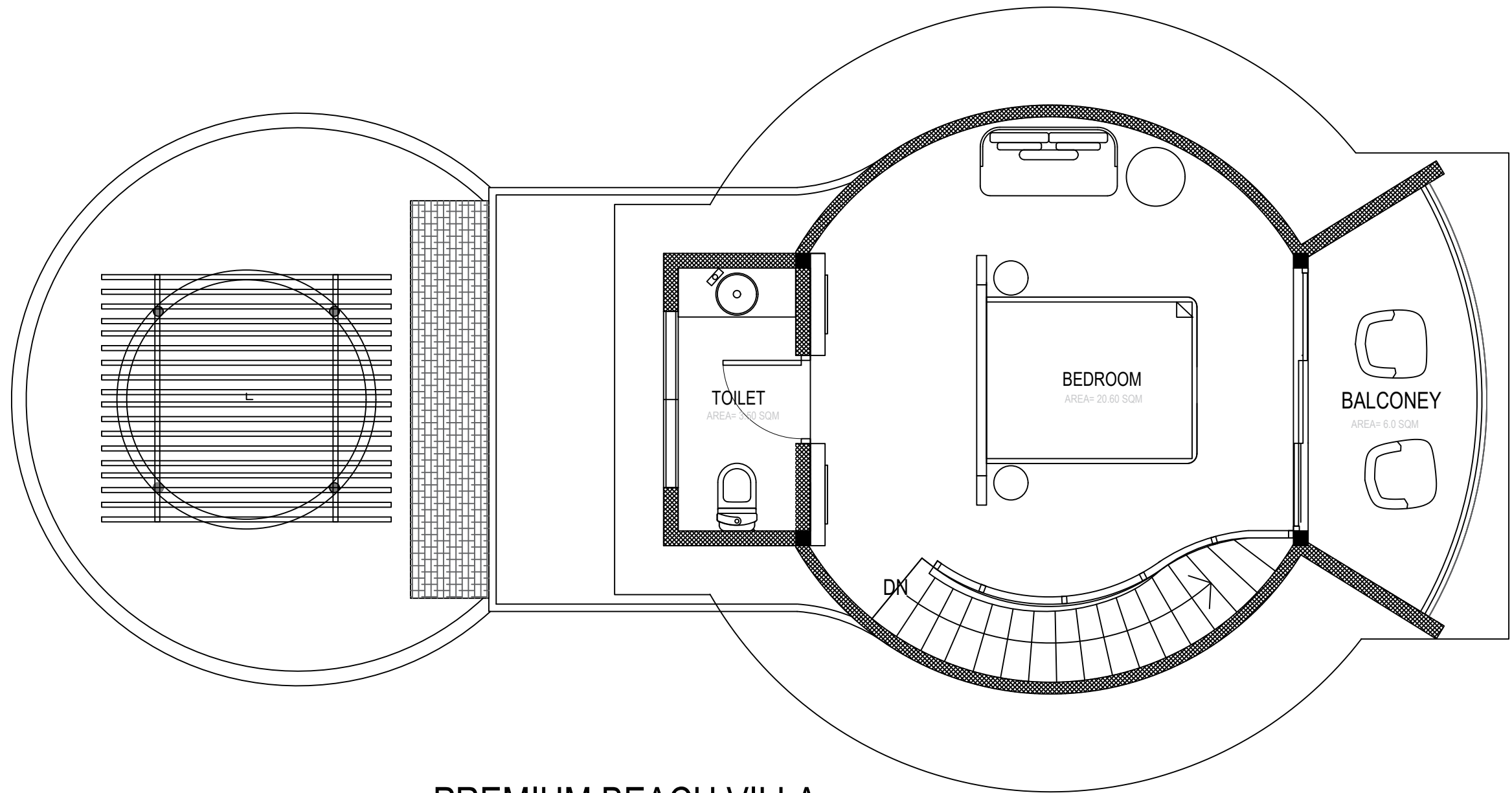
PREMIUM BEACH VILLA FIRST FLOOR
