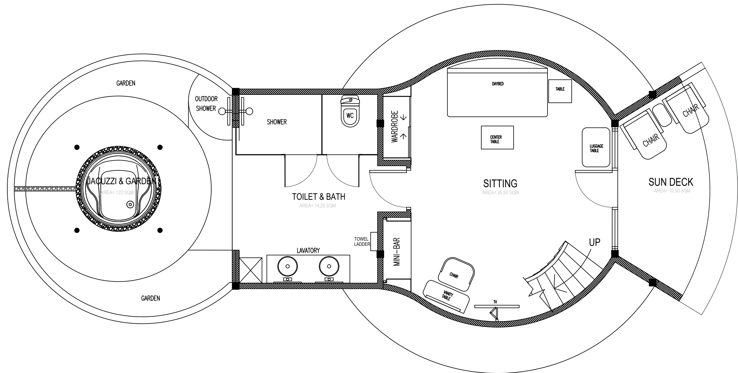
PREMIUM BEACH VILLA GROUND FLOOR
